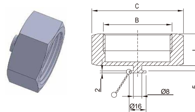
IDF-13HBN Hex.blank nut
