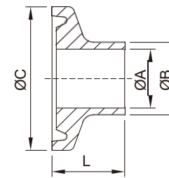
3A-1/2"~3/4" SMS-DN15~DN20 DIN-DN6~DN8 DIN(ISO)-DN6~DN10
