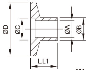
Weld Flange
