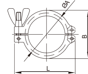
KF-Clamps
