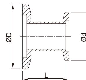
Straight Reducer
