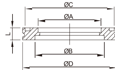
Weld Flange
