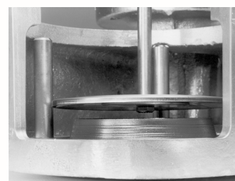
Pallet Assembly in Relieving Position
